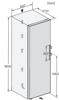
FNS4782E N, FNS4782D N, FNS4882D N, FNS4383E N, Nordics, installation sketch
